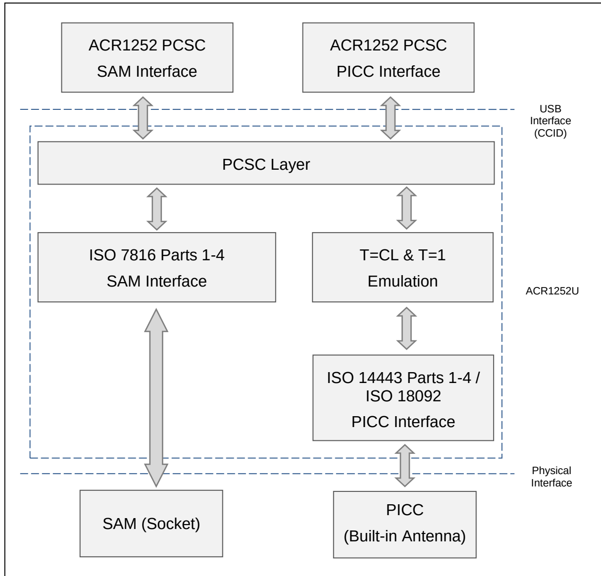
Figure 1: ACR1252U Architecture
